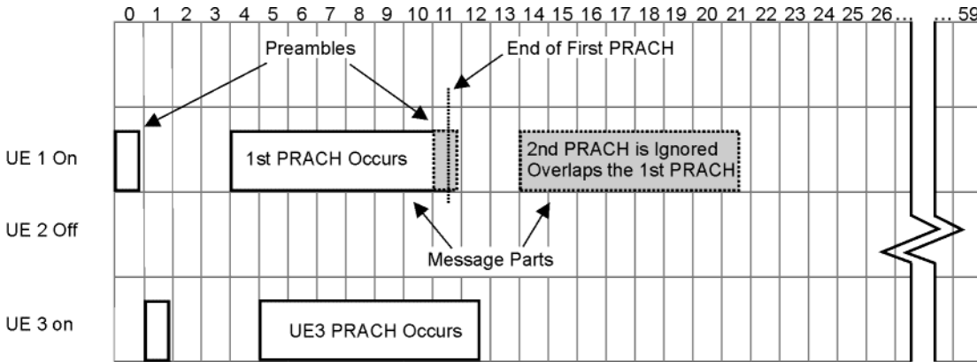
Figure 16-21 Transmitting PRACHs
